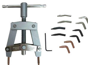
LANG87 H.D. Pliers with Tip Kit Internal & External 3.5" - 7". Compound screw lever for easy installation and removal of extra large retaining rings. Sale $131.19 Tool Club $104. 95
